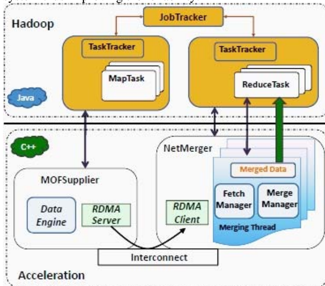
Fig 2: Hadoop structure
