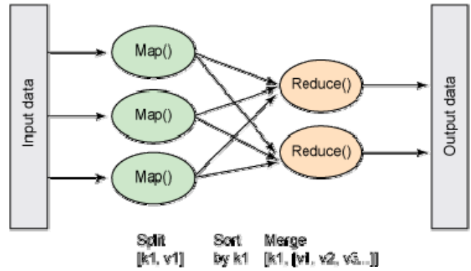
Fig 3: Map reduce
